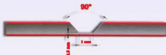
V-Shaped Groove for 90° folding
