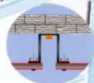
Exposed Riveted Fixing
